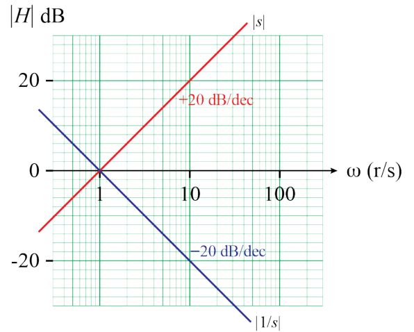
Fig. 2. Magnitude for s or 1/s .
