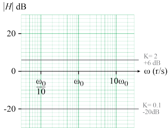
Fig. 1. Magnitude for constant multiplier.
