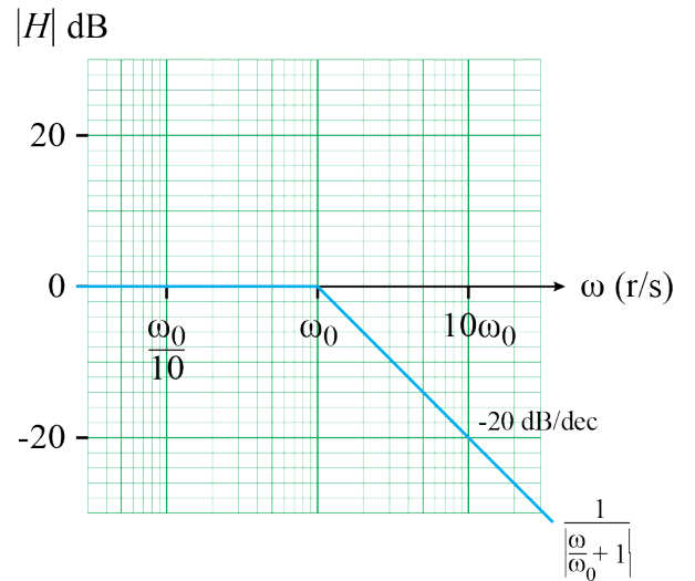
Fig. 4. Magnitude for real pole at \omega_0 .
