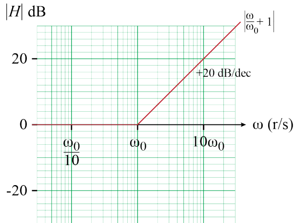
Fig. 3. Magnitude for real zero at \omega_0 .
